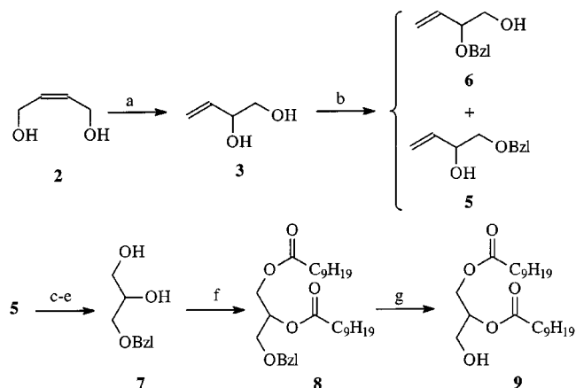
Scheme 1. Racemic synthesis of 1,2-diglyceride 9 by the benzylation pathway. Reagents and conditions: (a) H_2SO_4 , HgSO_4 , H_2O , microwave oven. – (b) BzI , NaH , Bu_4NI , THF . – (c) Pivaloyl chloride, CH_2Cl_2 , Pyr , 0^\circ C to room temp. – (d) O_3 , Me_2S , CH_2Cl_2 , -78^\circ C . – (e) NaBH_4 , CH_2Cl_2 , EtOH , 0^\circ C . – (f) Decanoic acid, DCC , DMAP , Et_2O . – (g) 5% Pd/C , H_2 , EtOH .
