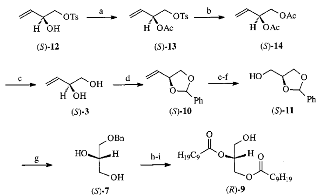
Scheme 3. Enantioselective synthesis of chiral 2,3-diglyceride ( R )- 9 . Reagents and conditions: (a) Acetyl chloride, CH 2 Cl 2 , Pyr, 0 °C. – (b) Caesium acetate, DMSO, DMF. – (c) K 2 CO 3 , MeOH, H 2 O. – (d) PhCHO, p -TsCOH, PhMe, reflux. – (e) O 3 , Me 2 S, CH 2 Cl 2 , –78 °C. – (f) NaBH 4 , CH 2 Cl 2 , EtOH, 0 °C. – (g) DIBALF, Et 2 O, 0 °C to room temp. – (h) Decanoic acid, DCC, DMAP, Et 2 O. – (i) 5% Pd/C, H 2 , EtOH.
