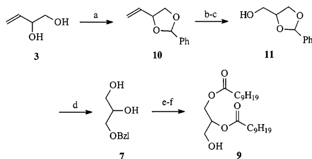
Scheme 2. Racemic synthesis of 1,2-diglyceride 9 by the benzylidene acetal pathway. Reagents and conditions: (a) PhCHO , p-TsCOH , PhMe , reflux. – (b) O_3 , Me_2S , CH_2Cl_2 , -78^\circ C . – (c) NaBH_4 , CH_2Cl_2 , EtOH , 0^\circ C . – (d) Decanoic acid, DCC , DMAP , Et_2O . – (e) 5% Pd/C , H_2 , EtOH .
